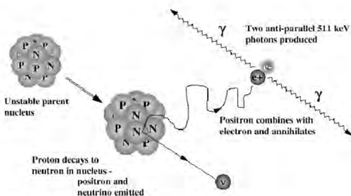
Figure 1.1. Positron emission and annihilation.
